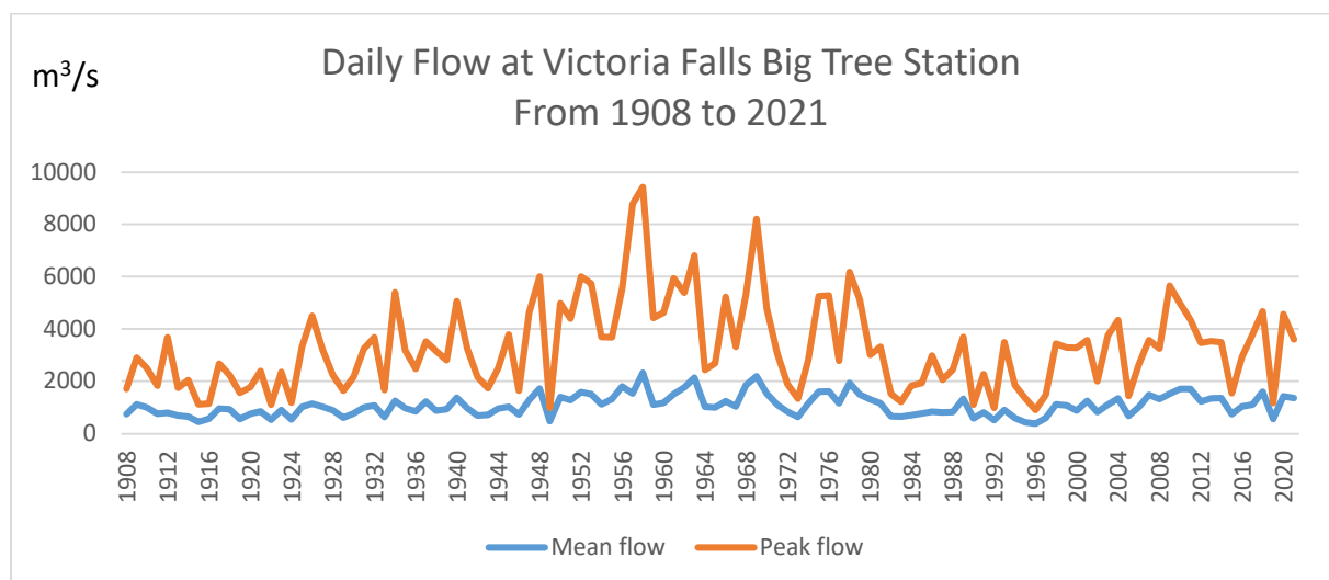
Figure 7: Historical peak and mean Zambezi flows at Victoria Falls between 1908 and 2021 – graph derived from annual flow data received from ZRA.
